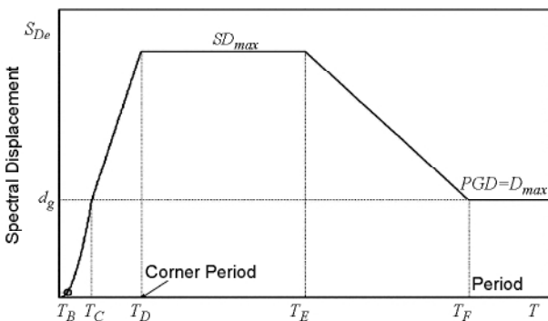
Figure 1. Elastic displacement spectrum [2].
